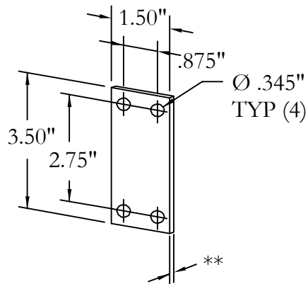
Standard Multi-Hanger Inline Spacer
