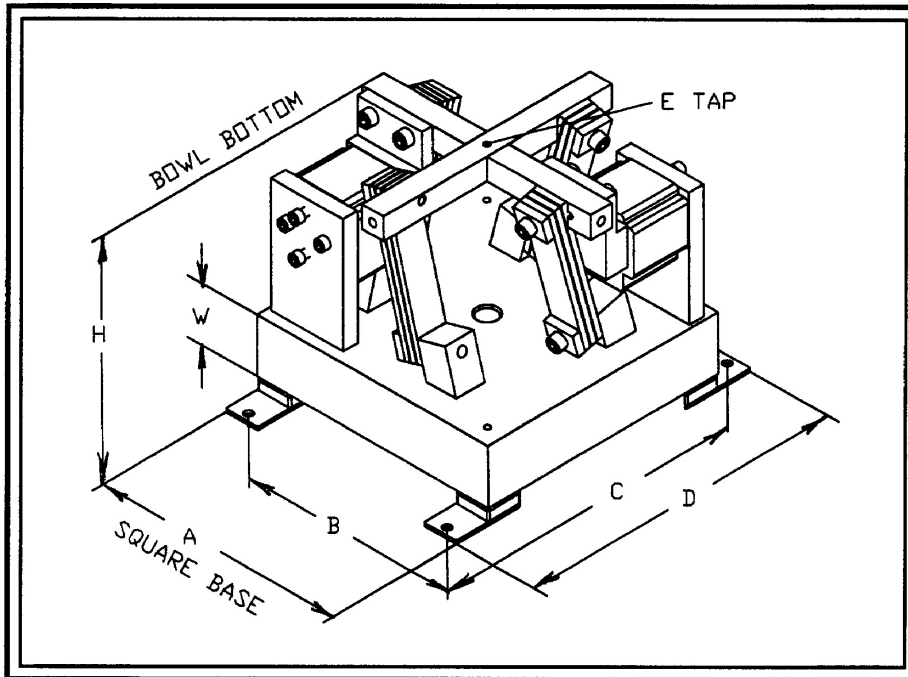
DRIVE BASE BASIC DIMENSIONS
